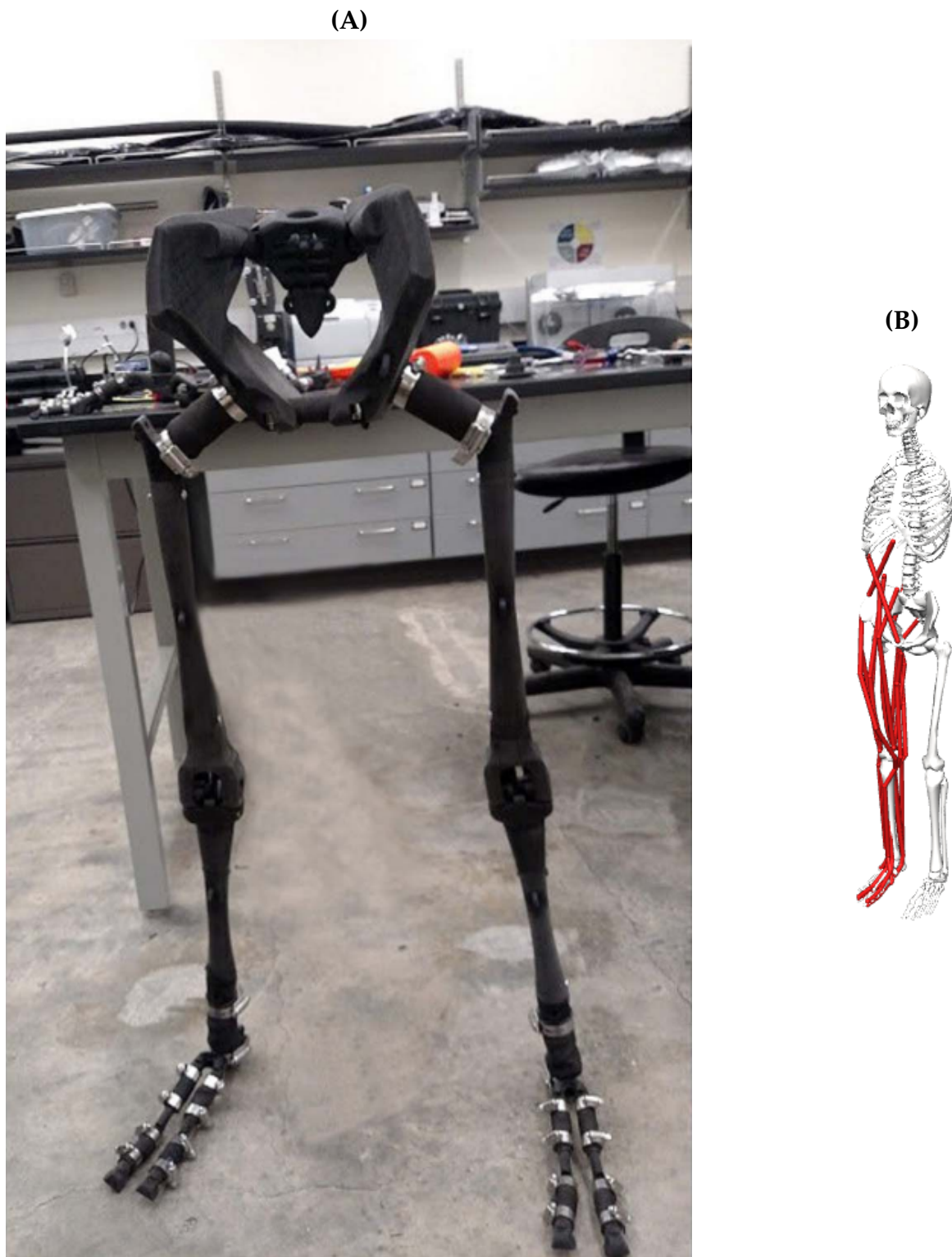
Figure 2.5: (A) The laboratory bipedal skeleton (actuators not installed in this view). (B) The Gait2392-derived OpenSim model used to develop its muscle routing; the view exposes the retained lower-limb musculotendon paths used as biomechanical design references [Bolen and Hunt, 2019, Morrow et al., 2020].
