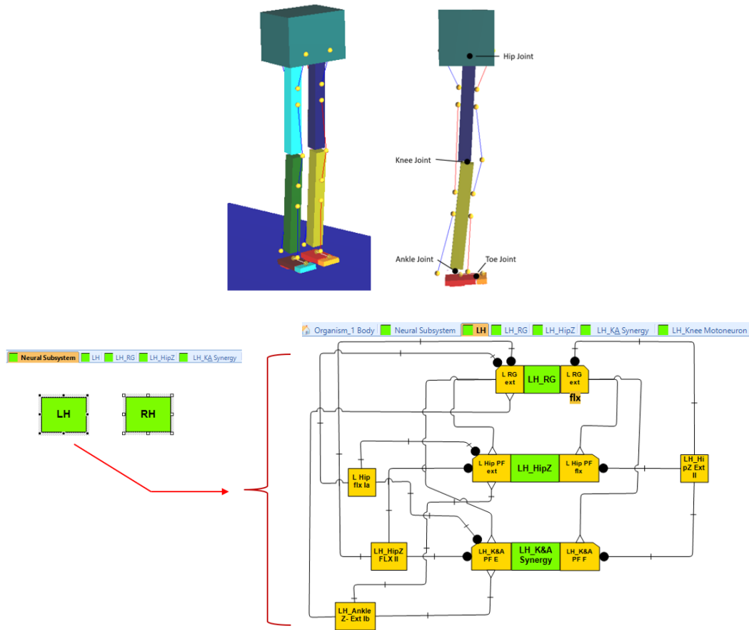
Figure 3.8: AnimatLab model and architecture illustrations. Top: the segmented walker and labeled hip, knee, ankle, and toe joints. Bottom: the left/right subsystem organization and an expanded view of the left-side rhythm-generator, hip, and knee–ankle modules. These architectural views describe model organization and are not snapshots of the phase-1 trajectory.
